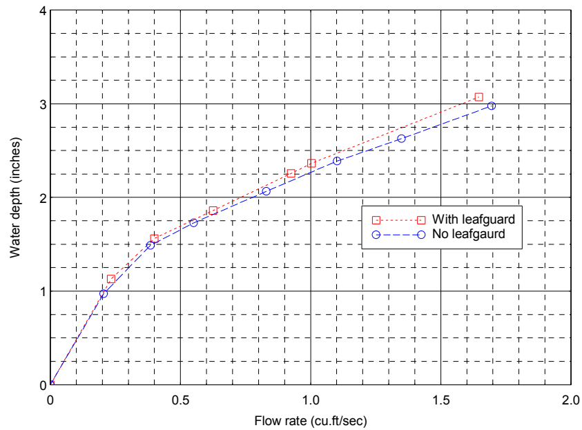
Figure 2, Rating curve (ft³/s format)
