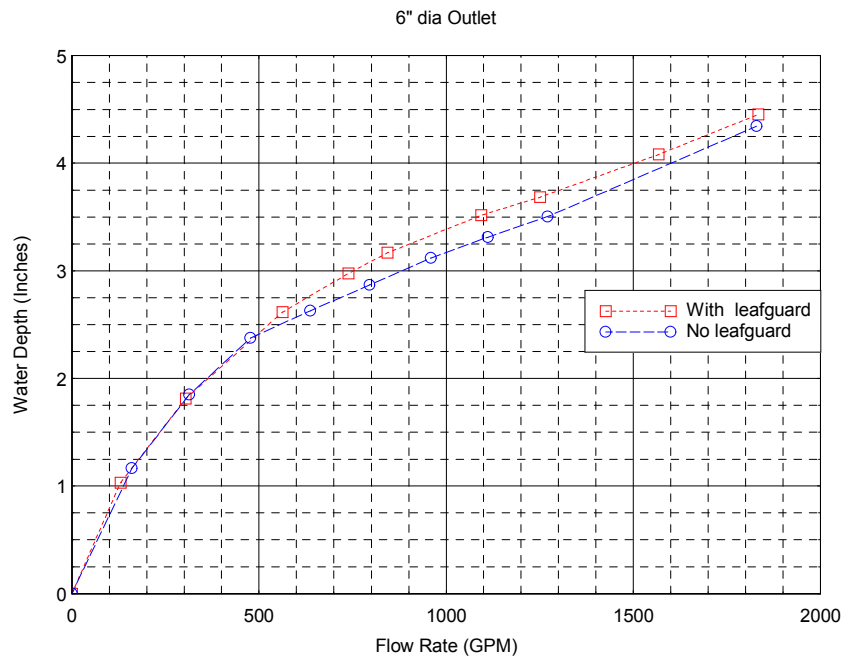
Figure 1, Rating curve (GPM format)
