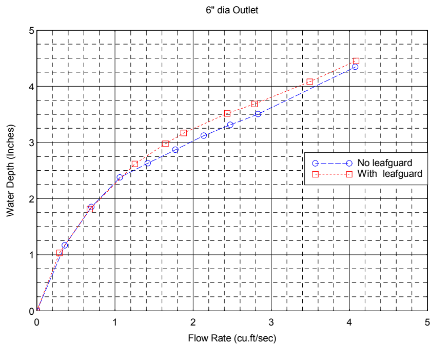
Figure 2, Rating curve (ft 3 /s format)
