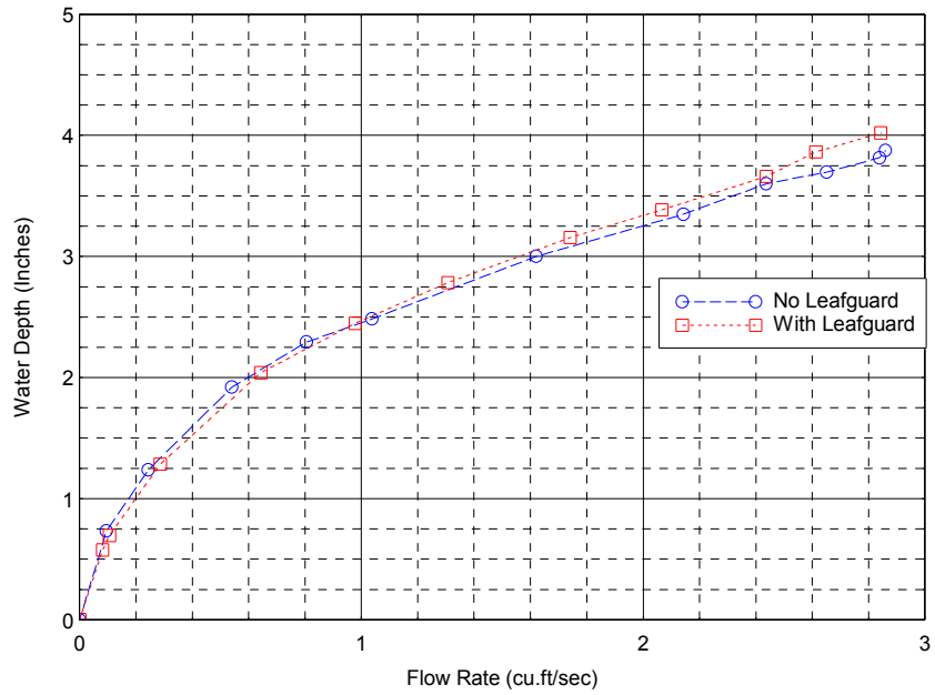
Figure 2, Rating curve (ft 3 /s format)
