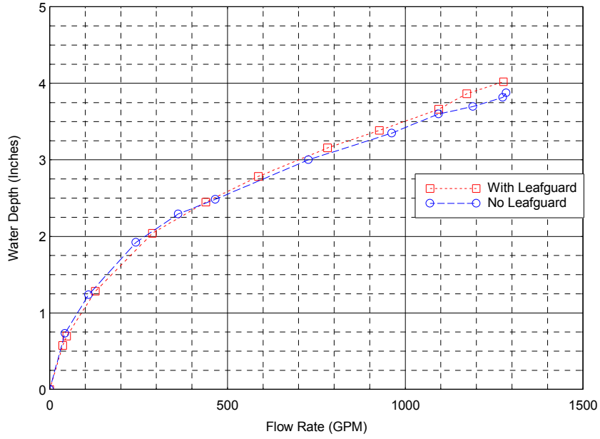
Figure 1, Rating curve (GPM format)
