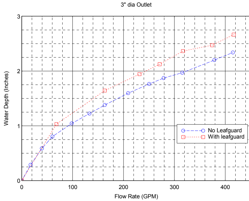
Figure 1, Rating curve (GPM format)
