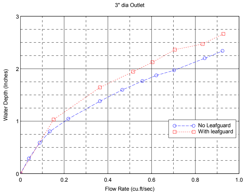
Figure 2, Rating curve (ft 3 /s format)
